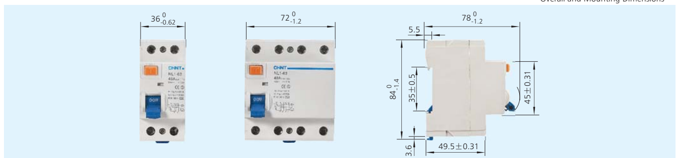
Overall and Mounting Dimensions
